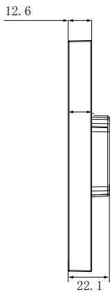
② RIGHT VIEW
